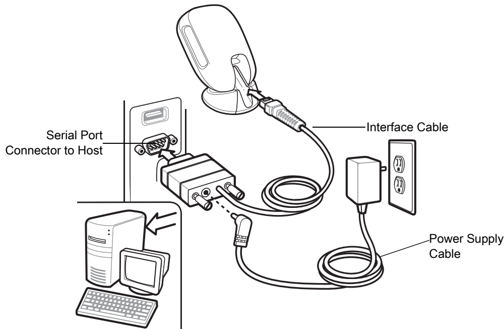
Figure 20 RS-232 Connection
